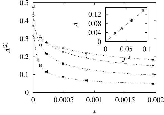
Fig. 2. Dependences of \Delta^{(2)} on x (= 1/2L^2) for \alpha = 0.5 and L = 16 \sim 80 . Points denote the QMC data for J' = 0.3, 0.25, 0.2, and 0.15 from top. The lines show the fitting function \Delta^{(2)}(x) . In the inset the J'^2 dependence of the spin gap is shown. The line with the slope of 1.5 is the guide to eyes.
